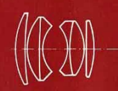
S1 50 mm f 1.8
