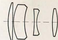
TYPE Y12 90 mm f 2.5
