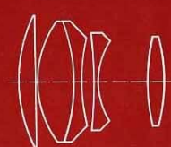
P1 90 mm f 1.8
