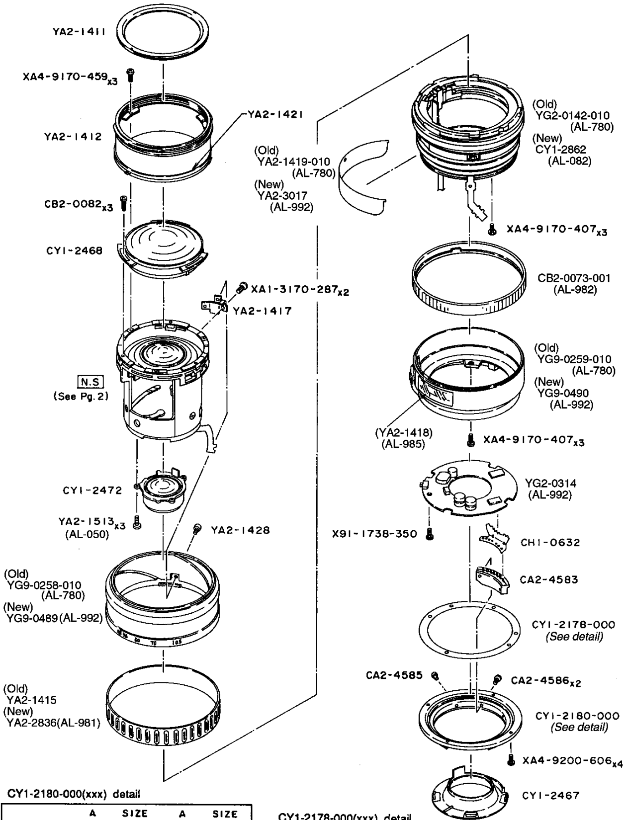
CY1-2178-000(xxx) detail
