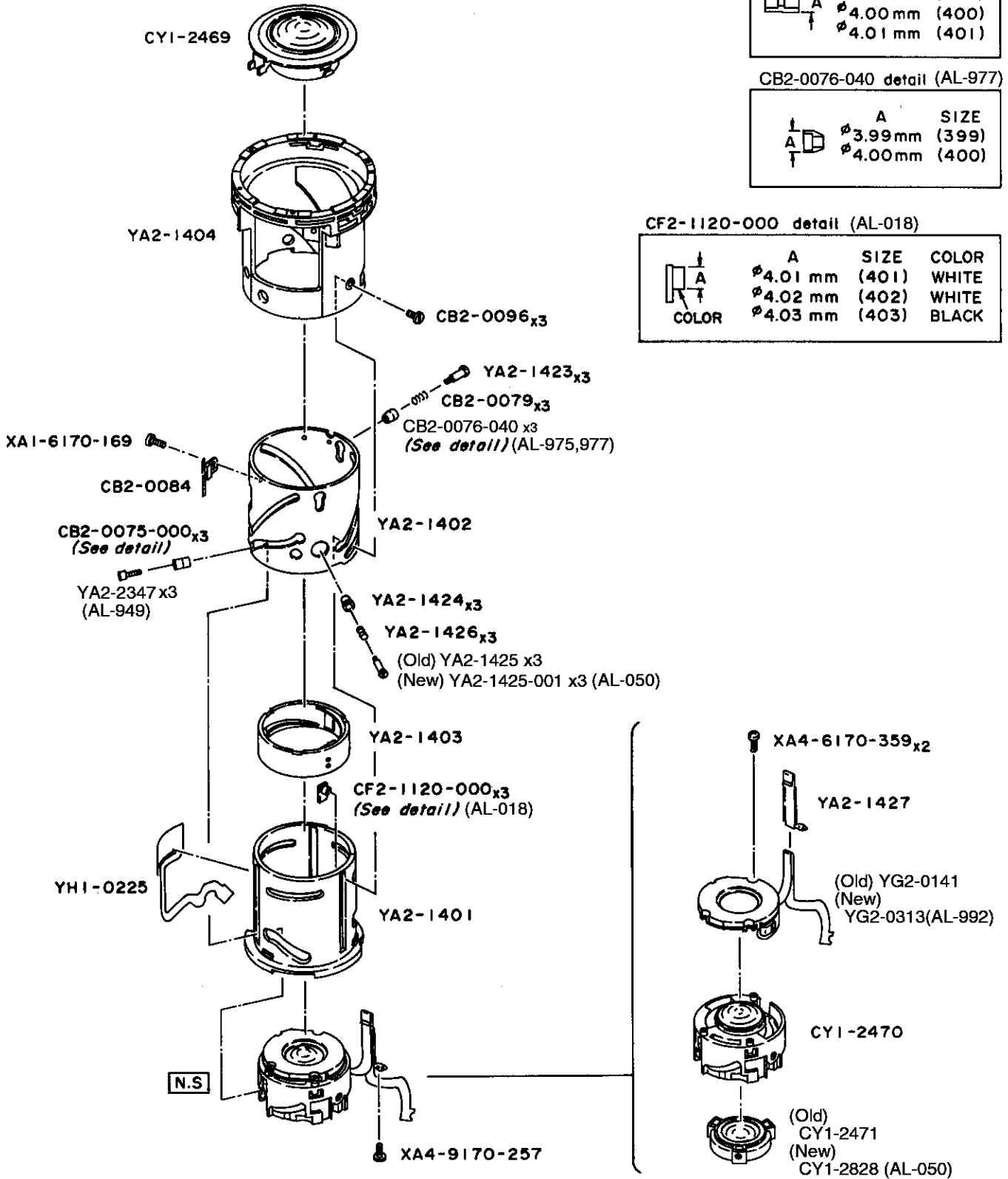
CB2-0075-000 detail
