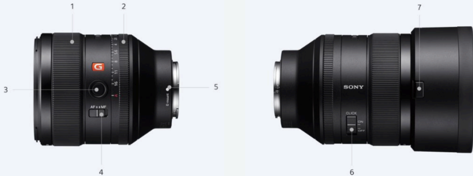
1. Focusing ring / 2. Aperture ring / 3. Focus hold button / 4. Focus mode switch / 5. Mounting index / 6. Aperture click switch / 7. Hood release button
